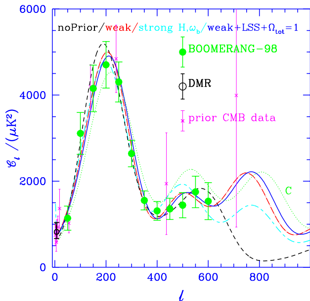
FIG. 1: CMB angular power spectra, \mathcal{C}_\ell \equiv \ell(\ell + 1)\langle |T_{\ell m}|^2 \rangle / (2\pi) , where the T_{\ell m} are the multipole moments of the CMB temperature. The closed (green) circles show the B98 data. The magenta crosses are a radical compression of all the data prior to B98 into optimal bandpowers [2, 3, 4], showing the qualitative improvement provided by B98 except in the \ell \lesssim 20 DMR regime, where the COBE data are represented as a single bandpower (open black circle). (Note that the B98 and prior CMB points at \ell = 150 lie on top of each other.) The smooth curves depict power spectra for several maximum likelihood models with different priors chosen from Table I, with (\Omega_{\text{tot}}, \omega_b, \omega_c, \Omega_\Lambda, n_s, \tau_c) as follows: P1, short dashed line, (1.3, 0.10, 0.80, 0.6, 0.80, 0.025); P4, dot-dashed line, (1.15, 0.03, 0.17, 0.4, 0.925, 0); P8, short-long dashed line, (1.05, 0.02, 0.06, 0.90, 0.825, 0); P11, solid line, (1.0, 0.03, 0.17, 0.70, 0.95, 0.025). These curves are all reasonable fits to the B98+COBE data. For comparison, we plot a H_0 = 68 , \Omega_\Lambda = 0.7 “concordance model” which does not fit (dotted line labelled C), with parameters (1.0, 0.02, 0.12, 0.70, 1.0, 0).
