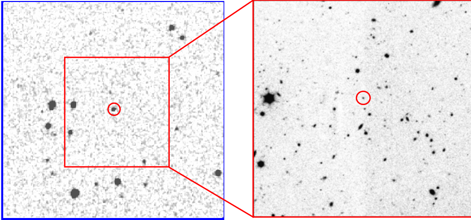
Figure 6. An example of a serendipitously discovered optical transient event from DPOSS. The left panel shows a portion of a DPOSS F plate image with an r \sim 18.5 magnitude, starlike object circled. The object was selected due to its apparent peculiar color (bright in r , extremely faint in the other two DPOSS bands); however, this was simply a consequence of the plates taken at different times, with one of them catching it in a bright state. The right panel shows a portion of the corresponding Keck R band image. The DPOSS transient was positionally coincident with an R \sim 24.5 magnitude galaxy, with an estimated probable z \sim 1 . At such a redshift, this object would have been a few hundred times brighter than a supernova at its peak. It may be an example of a GRB “orphan afterglow”, or possibly some other, new type of a transient.
