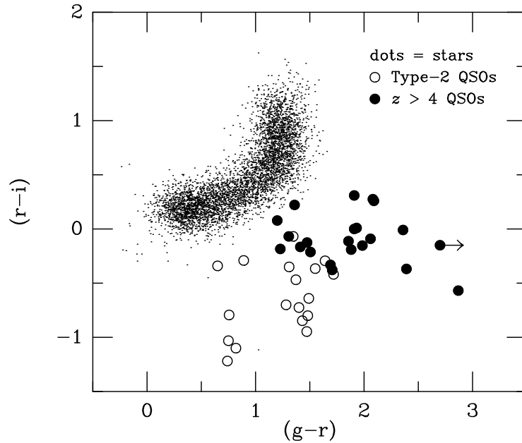
Figure 1. A representative color-color plot for objects classified as PSF-like in DPOSS. The dots are normal stars with r \sim 19 mag. Solid circles are some of the z > 4 quasars, and open circles are some of the type-2 quasars found in this survey. While quasars are morphologically indistinguishable from ordinary stars, this color parameter space offers a good discrimination among these types of objects. Similar methodology is now also used to discover brown dwarfs in SDSS and 2MASS.
