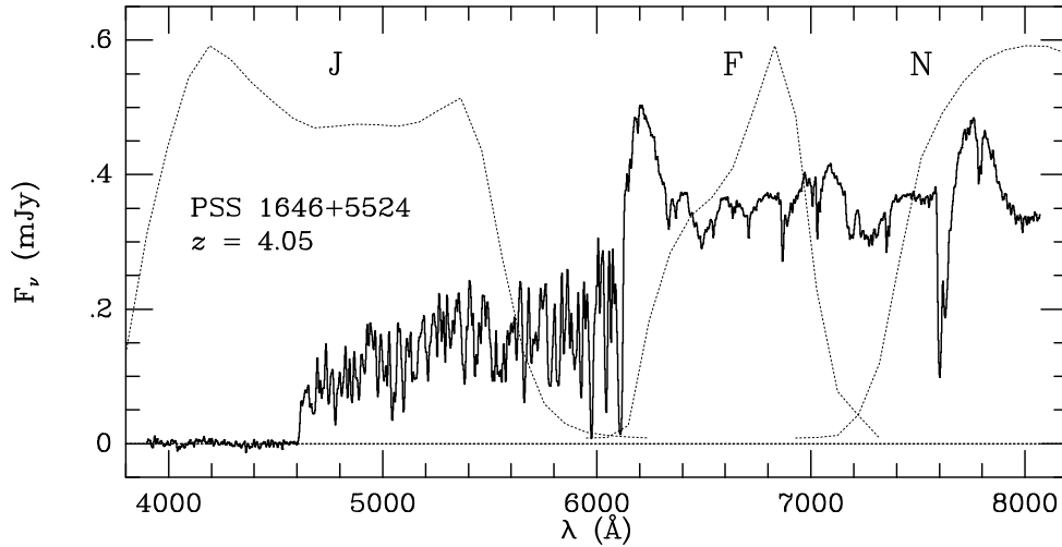
Figure 2. A spectrum of a typical z > 4 quasar, with the DPOSS bandpasses shown as dotted lines. The mean flux drop blueward of the Ly \alpha line, caused by the absorption by Ly \alpha forest and sometimes a Lyman-limit system, gives these objects a very red ( g - r ) color, while their intrinsic blue color is retained in ( r - i ). This places them in the portion of the color parameter space indicated in Figure 1.
