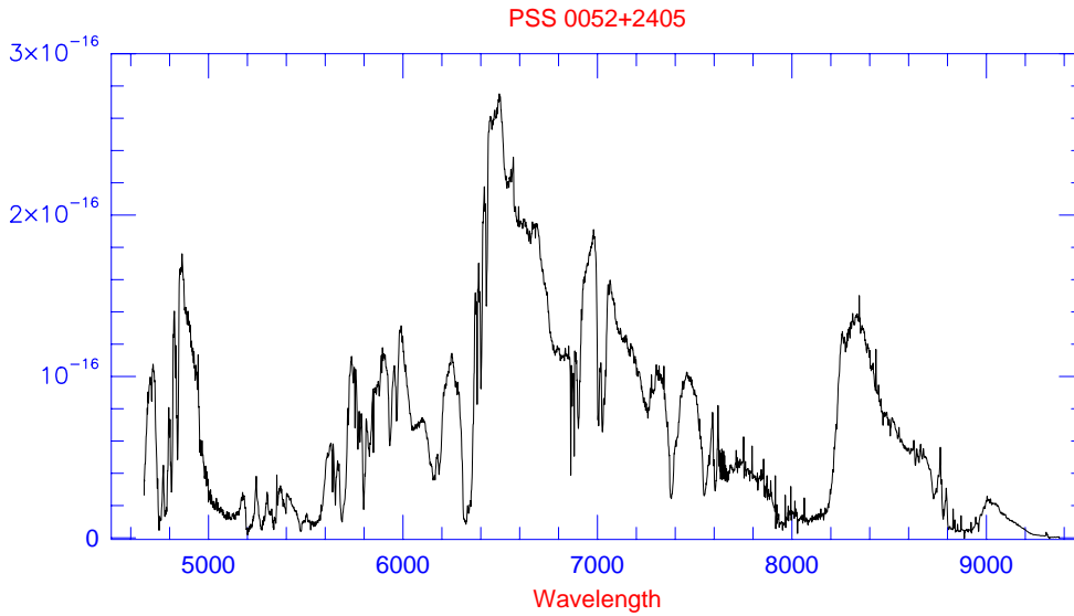
Figure 5. A spectrum of another peculiar object, PSS 0052+2405, obtained at Keck. This object was also initially selected as a high- z quasar candidate. Its nature is still uncertain, but it may be another example of a peculiar BAL QSO — or something completely different.
