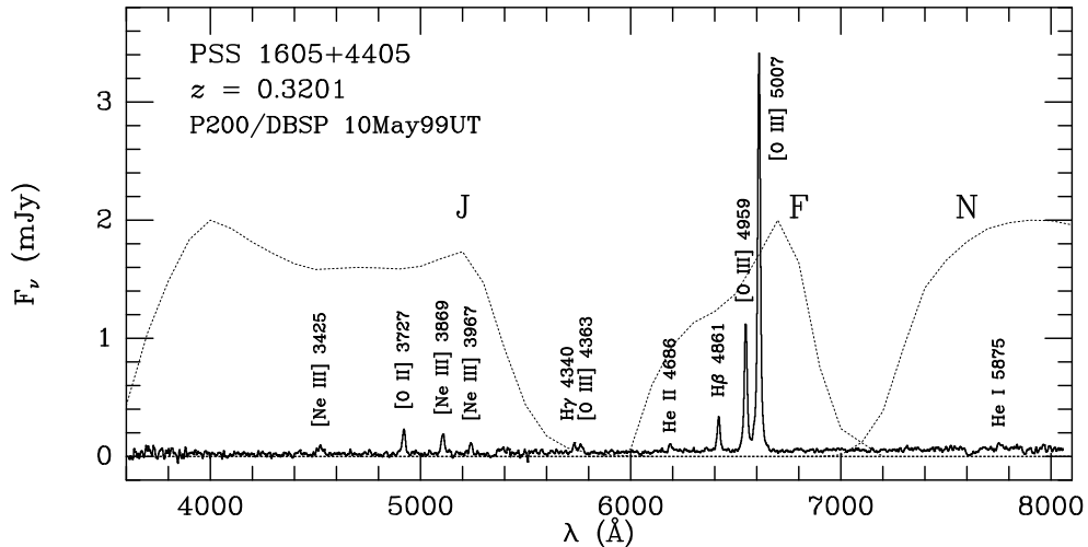
Figure 3. A spectrum of a typical type-2 quasar, with the DPOSS bandpasses shown as dotted lines. The presence of the strong [O III] lines is the r band places such objects in the portion of the color parameter space indicated in Figure 1.
