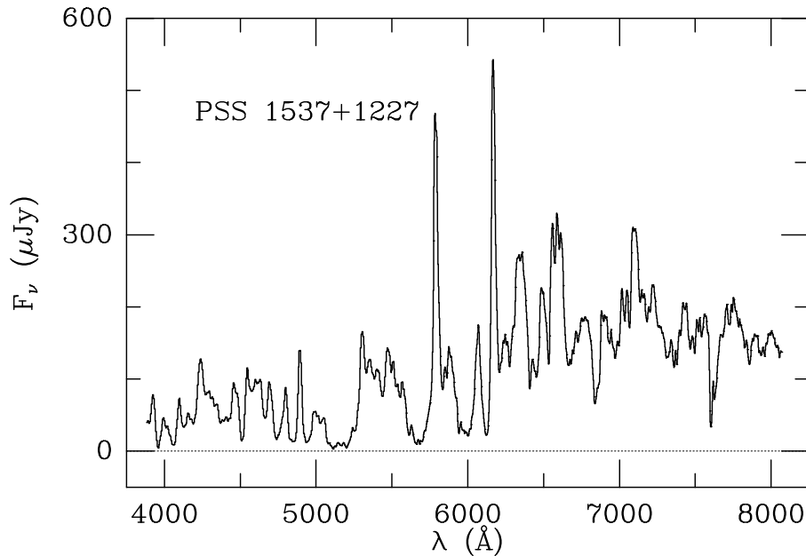
Figure 4. A spectrum of a peculiar object PSS 1537+1227, obtained at Palomar. The object was initially selected as a high- z quasar candidate due to its colors, in a manner illustrated in Figure 1. It turned out to be an extreme case of a rare type of a low-ionization, Fe-rich, BAL QSO, at z \approx 1.2 . A prototype case (but with a spectrum not quite as extreme as this) is FIRST 0840+3633, discovered by Becker et al. (1997).
