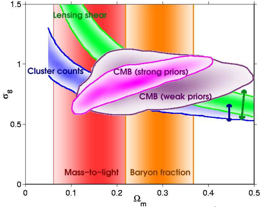
Figure 1.4: Various constraints shown in the \Omega_m - \sigma_8 plane. [Figure provided by Sarah Bridle; see also Ref. 45.] See full-color version on color pages at end of book.
