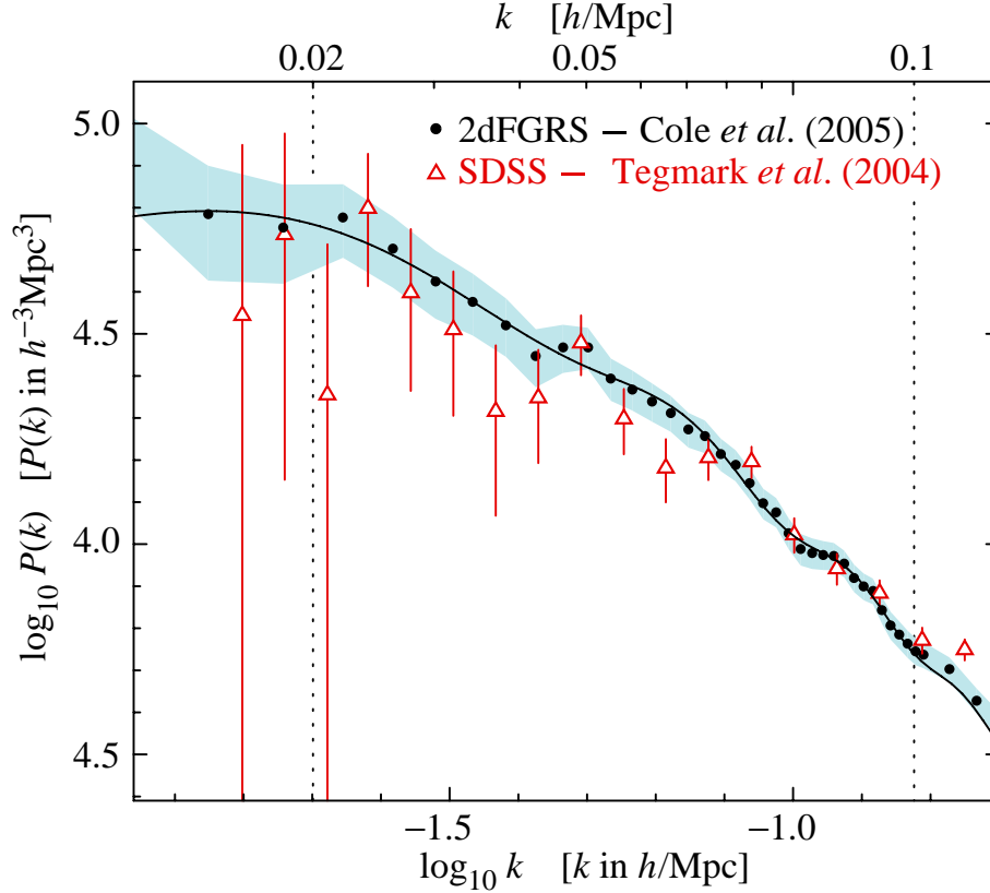
Figure 1.3: The galaxy power spectrum from the 2dF galaxy redshift survey [23] compared with that from SDSS [25], each corrected for its survey geometry. The 2dFGRS power spectrum (with distances measured in redshift space) is shown by solid circles with one-sigma errors shown by the shaded area. The triangles and error bars show the SDSS power spectrum. The solid curve shows a linear-theory \Lambda CDM model with \Omega_m h = 0.168 , \Omega_b/\Omega_m = 0.17 , h = 0.72 , n = 1 and normalization matched to the 2dFGRS power spectrum. The dotted vertical lines indicate the range over which the best-fit model was evaluated. [Figure provided by Shaun Cole and Will Percival; see Ref. 23.]
