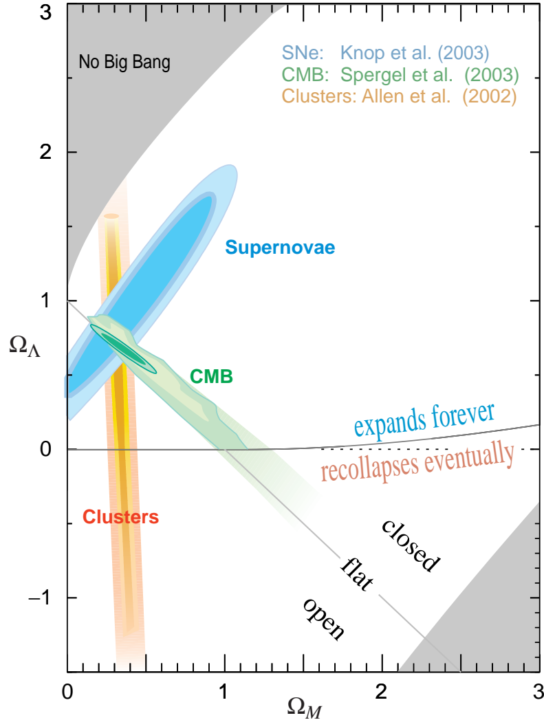
Figure 1.1: This shows the preferred region in the \Omega_m - \Omega_\Lambda plane from the compilation of supernovae data in Ref. 16, and also the complementary results coming from some other observations. [Courtesy of the Supernova Cosmology Project.] See full-color version on color pages at end of book.
