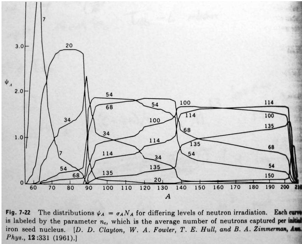
Fig. 17.— The distribution of heavy isotopes as a function of the neutron exposure. (Figure from chapter 7 of Clayton)
