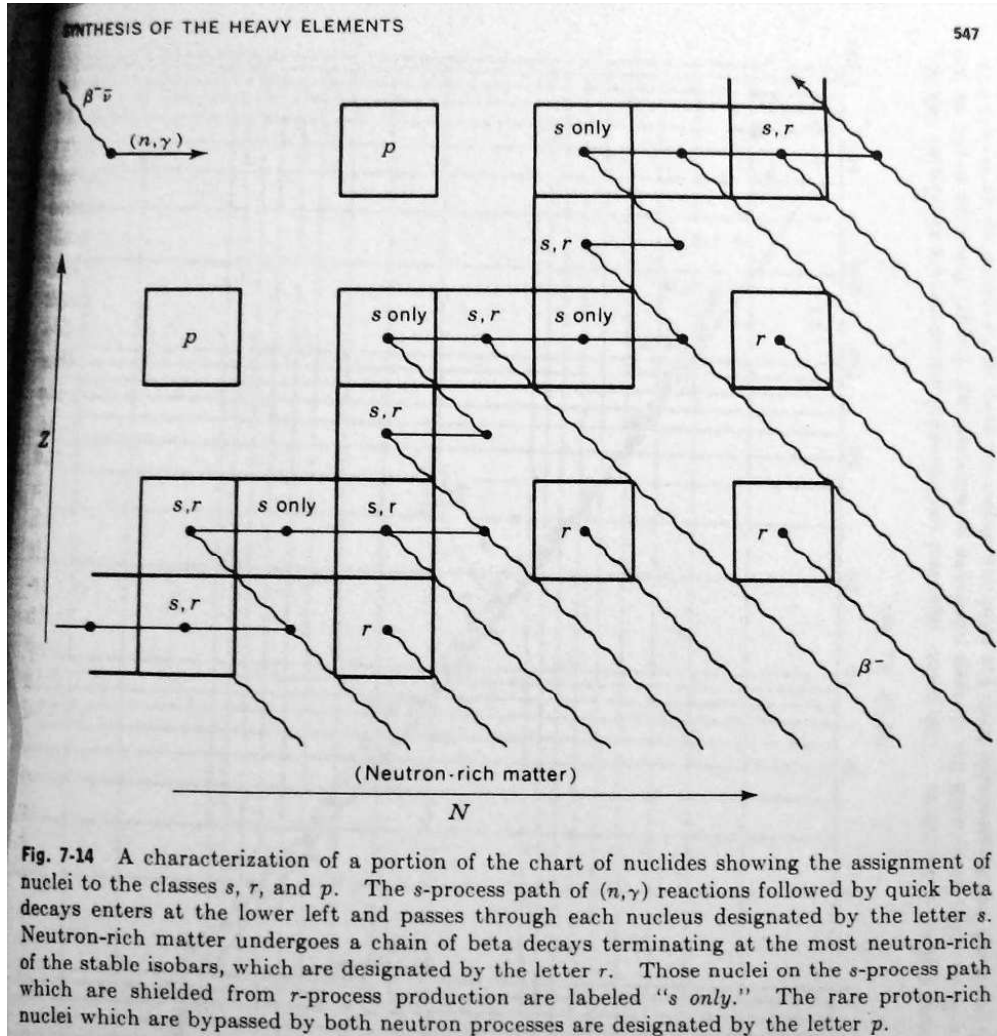
Fig. 15.— A schematic diagram of neutron number ( X ) versus atomic number ( Y ) showing the path of the s and the r process through the various isotopes. Wavy lines denote \beta decays. (Figure from chapter 7 of Clayton)
