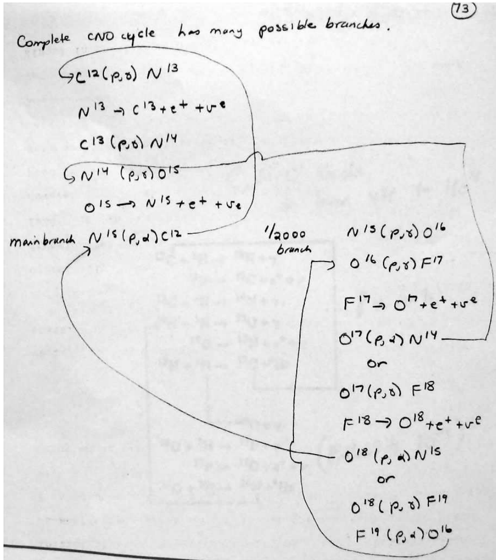
Fig. 9.— Examples of some side chains to the main CNO cycle. See also Table 6.2 of HKT.
