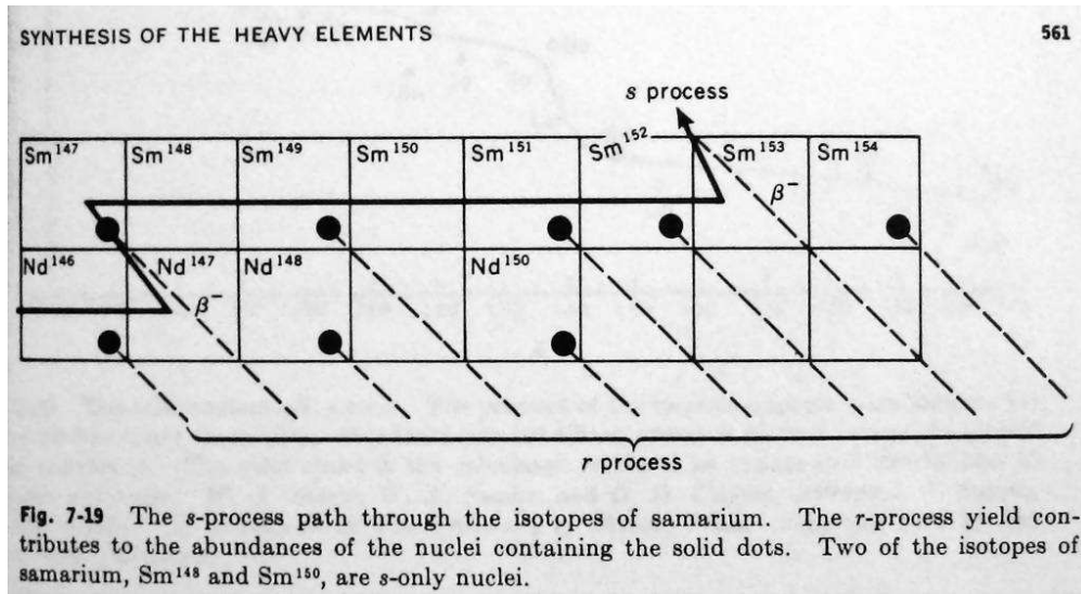
Fig. 16.— The s -process path through the isotopes of the rare earth samarium, with some contribution from the r -process in the case of certain specific isotopes. (Figure from chapter 7 of Clayton)
