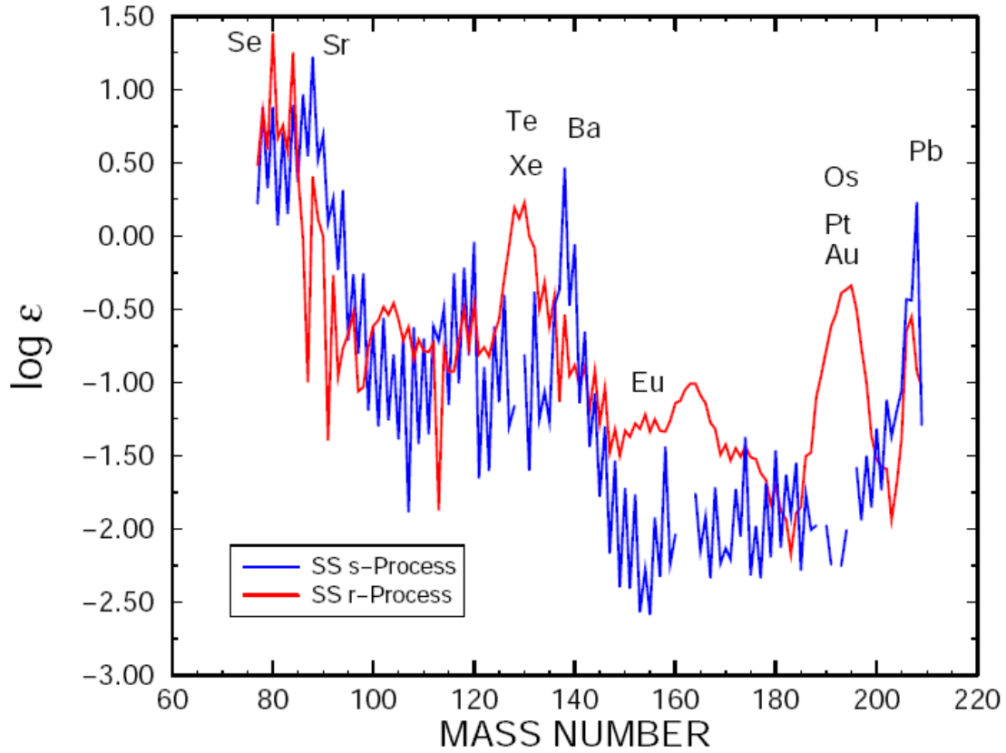
Fig. 13.— The s and r process isotopic abundances in the Sun, based on Kappeler et al (1989). These are on a scale such that \epsilon(H) = 10^{12}/\text{cm}^3 . Note the distinctive s -process peaks at A \approx 88, 138 and 208 , and the r -process peaks at A \approx 130 and 195 .
