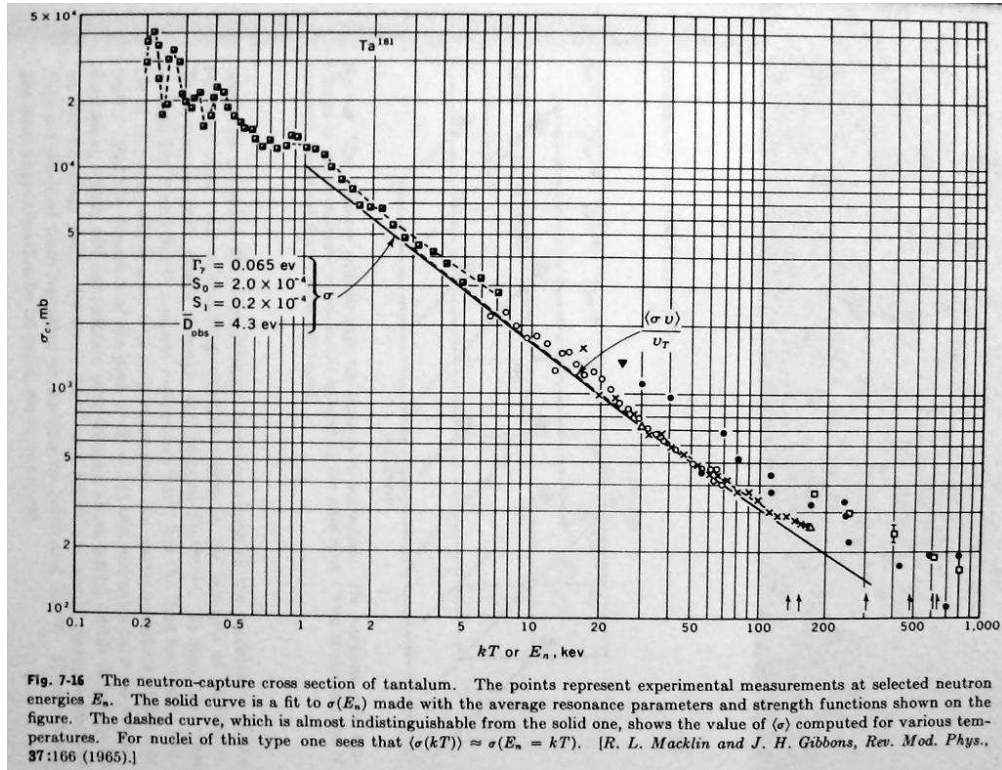
Fig. 14.— The neutron capture cross section as a function of energy for tantalum. (Figure from chapter 7 of Clayton)
