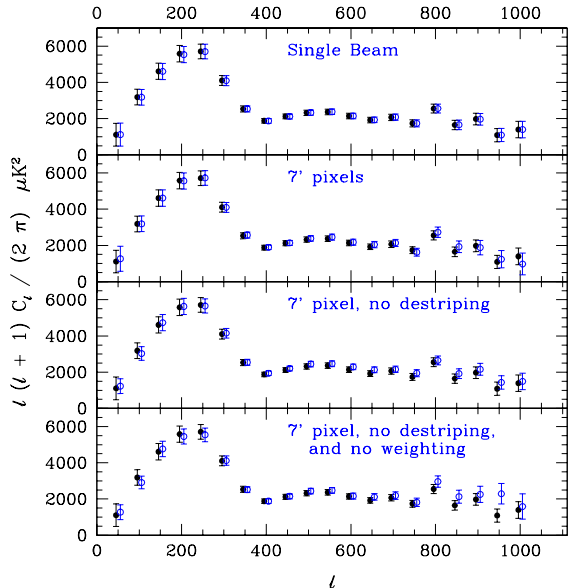
Fig. 3.— Angular power spectra derived from the FASTER pipeline. The solid black circles in each panel show the reference FASTER spectrum, which is derived from a 3.5' pixelized map using S+N weighting, spatially filtered as described in the text to remove constant-declination stripes. In the top panel the reference spectrum is compared with a spectrum derived using a single beam window function, as in MADCAP. The second panel shows the effect of using 7' pixelization. The third panel illustrates the effect of removing the constant declination stripes; the primary effect is to increase the error in the first bin. The bottom panel shows the result of using a uniformly weighted map and neglecting to remove the constant declination stripes. The top three panels show excellent agreement with the reference spectrum, while the bottom panel shows good agreement except at very high \ell .
