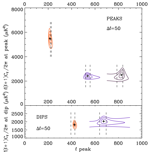
Fig. 11.— \Delta\chi^2 contours for the position and amplitude of peaks and valleys in the BOOMERANG MADCAP power spectrum. The contours are at \Delta\chi^2 = 2.3, 6.17, 11.8 , i.e. 68.3%, 95.4% and 99.7% confidence. The vertical dashed lines give the feature positions found using the cosmological database, and as given in Table 5. Similar results are obtained using the FASTER results.
