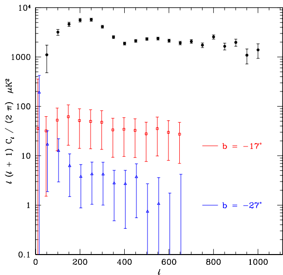
Fig. 8.— Angular power spectra of IRAS-correlated dust scaled to 150 GHz for two circles of radius 9^\circ centered at galactic latitudes of b = -17^\circ (red open squares) and b = -27^\circ (blue open triangles). Details of this analysis can be found in Masi et al. (2001). The FASTER CMB power spectrum (filled black circles) is shown for reference.
