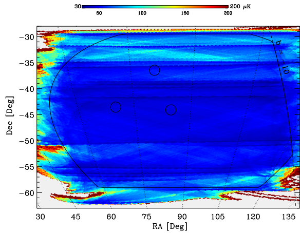
Fig. 1.— The sky covered by CMB observations; the color scale indicates the depth of coverage (diagonal component of the noise covariance matrix) in a 7' Healpix pixel, in the map produced by the MAD-CAP analysis described below. The region enclosed by the solid line is that used for the power spectrum estimation. The three circles show the locations of three bright known quasars; data within a 0.5^\circ radius of the quasars is not used in the power spectrum estimation.
