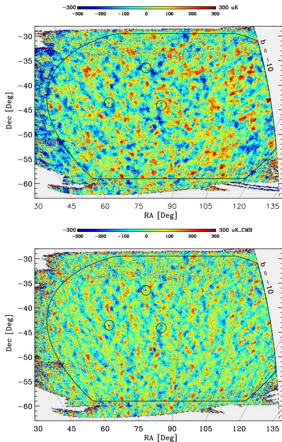
Fig. 2.— The maps of CMB temperature produced by MADCAP (top) and FASTER (bottom). For comparison, both maps are pixelized at 7' ; in practice we use a 7' ( 3.5' ) pixelization in the MADCAP (FASTER) analysis. The strikingly different appearance of the maps, with the MADCAP map preserving more information on large scales, illustrates some of the significant differences in the two analysis methods, as described in the text.
