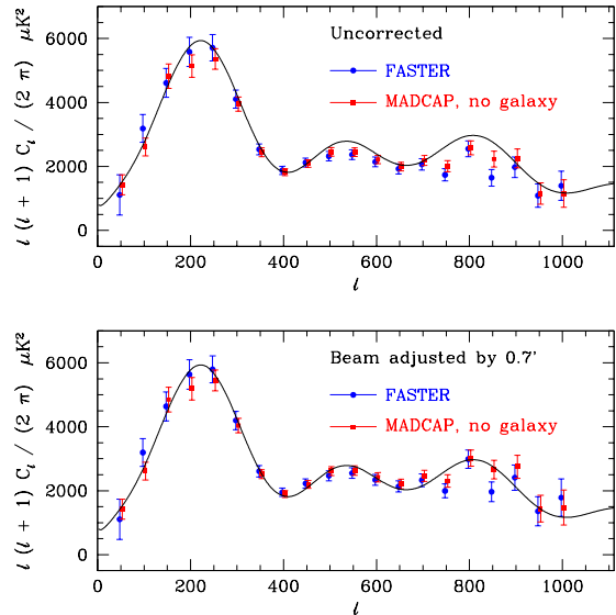
Fig. 10.— Final angular power spectrum results at 150 GHz, also given in Table 2. In both panels, the MADCAP results are shown as red squares, while the FASTER results are given as blue circles. The top panel shows the data of Table 2, along with the best-fit model from the weak-prior parameter estimation discussed below. In addition to the errors shown, there is a 10% uncertainty in the temperature calibration (20% in the temperature-squared units of this plot), and a beam uncertainty of 1.4' rms. In the bottom panel we have rescaled the data by changing the the beam window function by 0.5\sigma . This gives much better visual agreement with the model.
