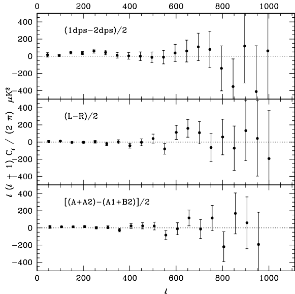
Fig. 6.— Difference map power spectra derived using FASTER. The top panel shows the (1\text{dps}-2\text{dps})/2 difference map results. The middle panel shows the result found by difference maps made from leftgoing scans and rightgoing scans, (L-R)/2 . The bottom panel is for a map made by differencing maps made by two channel combinations, [(A+A2)-(A1+B2)]/2 . While the latter two power spectra are relatively consistent with zero contamination, near \ell \sim 200 the (1\text{dps}-2\text{dps})/2 spectrum is not. This contamination is, however, much smaller than the statistical errors on the full CMB power spectrum in this \ell -region. The \chi^2 statistics of these spectra with respect to zero signal are given in Table 1.
