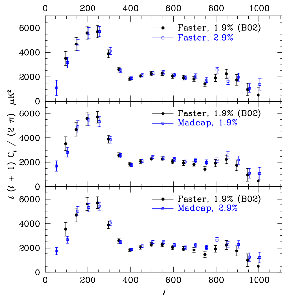
Fig. 7.— A comparison of the FASTER results of B02 (black filled circles) derived from 1.9% of the sky at 7' pixelization, with three new analyses (open blue squares in each panel). Top panel: the FASTER results of this paper (2.9% of the sky, 3.5' pixelization). Middle panel: a new MADCAP analysis of the B02 sky cut (1.9% of the sky, 7' pixelization). Bottom panel: the MADCAP results of this paper (2.9% of the sky, 7' pixelization). The agreement is generally very good, with the greatest variations at high \ell where noise, rather than cosmic variance, dominates the errors.
