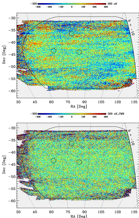
Fig. 4.— (1dps-2dps) difference maps, both at 7' pixelization to facilitate map comparisons by eye, for the region of sky where these scans overlap. The color scale is the same as for the previous figures. Note that the consistency test power spectra are calculated on these maps divided by two, (1\text{dps}-2\text{dps})/2 . Top panel: The MADCAP difference map. This map is not destriped, since in that pipeline the constant-declination stripes are ignored (by introducing a constraint matrix) in the derivation of the angular power spectrum. Bottom panel: The destriped FASTER difference map. Note that the MADCAP input time-stream contains additional low frequency information that is removed by an additional highpass filter in the FASTER pipeline.
