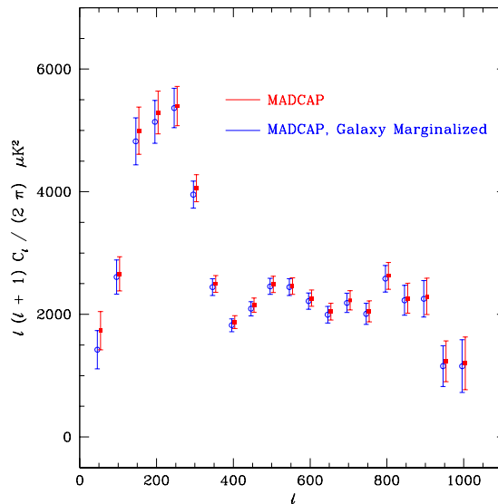
Fig. 9.— Galactic marginalization. The filled red squares show the results of the MADCAP analysis with marginalization over the constant-declination modes (to remove constant-declination striping). The open blue circles show the results after additional marginalization over two galactic templates, one of galactic dust and the other of galactic synchrotron emission. These lead to slight shifts in the power spectrum at low \ell , only significant in the first bin.
