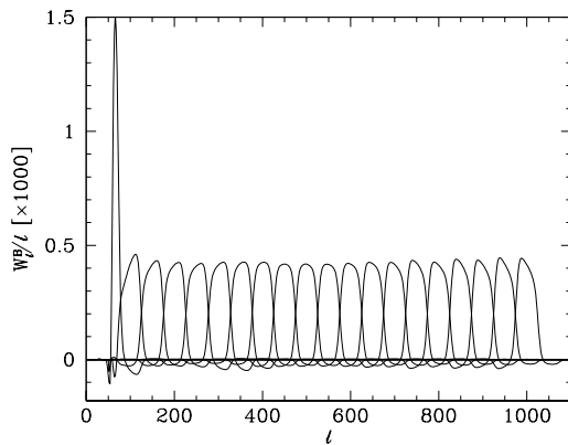
Fig. 12.— Window functions derived from the FASTER analysis. These window functions are used to relate a continuous theoretical model to the expected experimental band powers, a crucial step in parameter extraction. The functions are orthogonal, as a result of the top-hat binning assumed in the theory. The window for the first band shows how all the information is coming from the 50 < \ell < 76 region due to the sharp filtering applied (in the FASTER pipeline) to the timestream.
