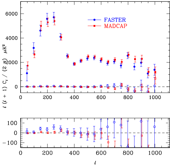
Fig. 5.— MADCAP and FASTER angular power spectra and (1dps-2dps)/2 difference map power spectra. Top Panel: the FASTER (filled blue circles) and MADCAP (filled red squares) angular power spectra, and their respective (1dps-2dps)/2 difference map power spectra (open symbols). The effects of constant-declination stripes have been removed in each of these analyses. Bottom panel: the difference map angular power spectra plotted on a magnified scale. There is a systematic effect near \ell \sim 200 in the FASTER power spectrum, which is absent in the MADCAP treatment. The level of these residuals is much smaller than the statistical errors on the full power spectrum, shown in the top panel.
