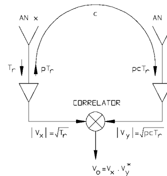
FIG. 2.—Cross talk between antennas in an array. T_r is the receiver noise, p is the correlation coefficient between the outgoing and receiver noises, pT_r is the outgoing receiver noise, which is correlated with T_r , and c is the coupling between the antennas. [If we transmit P , from antenna x and receive P_r at antenna y , then c = (P_r/P) .] The correlator is a complex multiplier (Thompson et al. 1986).
