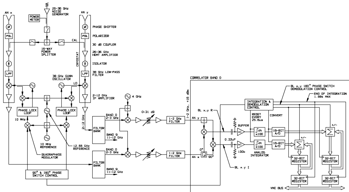
FIG. 8.—Signal processing in the CBI. Receiver details are shown for two antennas, x and y , and for band 0 of the downconverter. Correlator readout details are given for just one baseline ( x, y ) in band 0. “+” is a power splitter, and “Q” is a quadrature hybrid.
