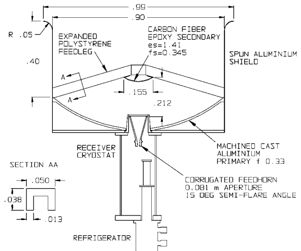
FIG. 7.—Cross section of a CBI antenna. Dimensions are in meters. “es” and “fs” are the eccentricity and focal length of the secondary. The top of the cryostat is bolted to the back of the antenna, and three tensioned struts run from the bottom of the cryostat to the antenna platform to stiffen the assembly.
