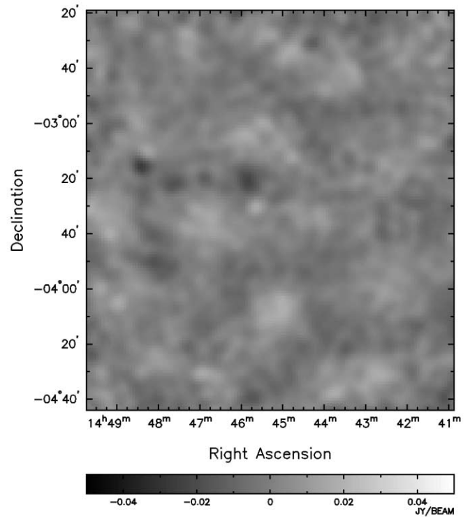
FIG. 12.—The 14^{\text{h}} field after removal of 63 point sources monitored by the OVRO 40 m telescope.
