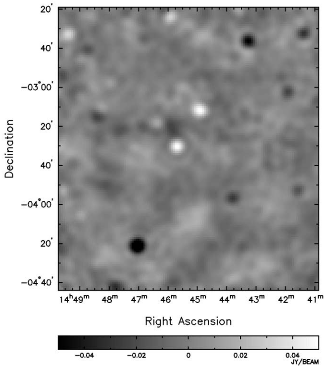
FIG. 11.—Mosaic of the 14^{\text{h}} CBI field made from 42 main-trail observations ( \sim 200 hr total observing time). All 10 frequency bands have been combined and the individual maps for each pointing center have been corrected for their primary beams. The mosaic was made pixel by pixel by summing the individual maps, weighting by the inverse variance. The rms noise in the mosaic varies from 1.5 \text{ mJy beam}^{-1} in the central area to \sim 5 \text{ mJy beam}^{-1} at the edges. The synthesized beamwidth varies from 4.7 to 5.3 (FWHM). The brightest point source in this image has a flux density of -96 \text{ mJy} .
