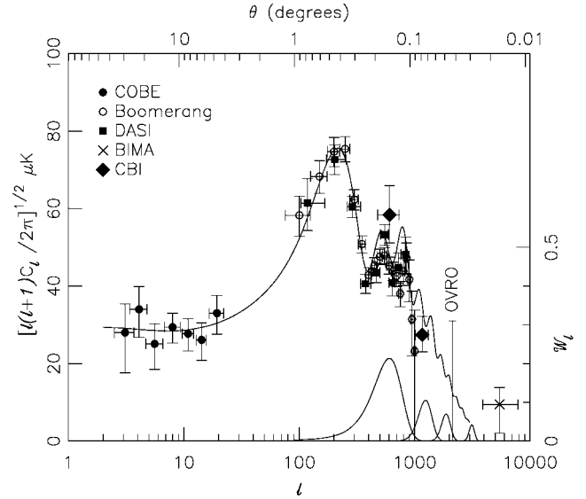
FIG. 1.—Some CMBR anisotropy measurements, shown with a \Lambda -CDM model with \Omega_0 = 1 , h = 0.70 , \Omega_b h^2 = 0.02 , and \Omega_\Lambda = 0.66 . At bottom are window functions for 1, 2, 3, and 5 m baselines in the CBI. The 1 m baseline is the shortest possible with our 0.9 m diameter antennas, and the tracking platform supports baselines up to 5.5 m. The window functions were obtained by computing the azimuthal average of (E * E)^2 using a Gaussian approximation to the aperture distribution for a single antenna, E_{\text{ant}}(r) = \exp - (2.3r/d)^2 . Data points are from COBE (Hinshaw et al. 1996), BOOMERANG (Netterfield et al. 2002), DASI (Halverson et al. 2002), BIMA (Dawson et al. 2001), and CBI (Padin et al. 2001b). The upper limit (95% confidence) is from OVRO (Readhead et al. 1989). The model was computed using CMBFAST (Seljak & Zaldarriaga 1996, 1997; Zaldarriaga, Seljak, & Bertschinger 1998).
