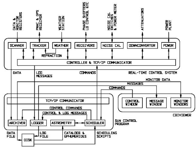
FIG. 10.—The CBI control system.
