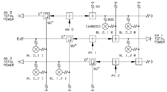
FIG. 9.—Architecture of the CBI correlator. This diagram shows a multiplier array for just three antennas. The CBI correlator uses a similar, but larger, array with 13 antenna inputs and 156 multipliers. The antenna inputs are along the diagonal, and for a square array, the path lengths to the two inputs of a multiplier are the same.
